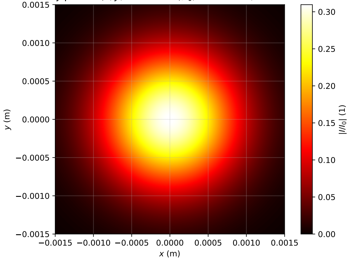
Intensity profile I(x, y, z = 3.184m)/I_0 , P_{in}=0.1P_{cr} , artificial time
